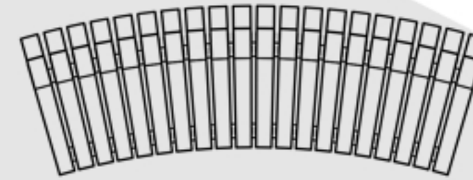
Plateu Seat - Curved Front Radius : 3500mm Front Radius Length : 1980mm Curve Type : Concave Timber 580mm x 120mm Taper : 80mm - 93mm
