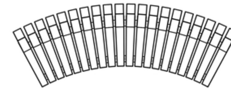
Plateu Seat - Curved Front Radius : 2000mm Front Radius Length : 1980mm Curve Type : Concave Timber 580mm x 120mm Taper : 80mm - 103mm
