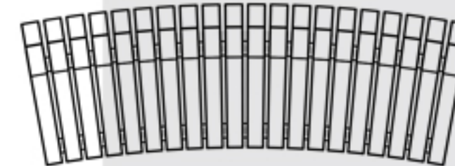
Plateu Seat - Curved Front Radius : 5500mm Front Radius Length : 1980mm Curve Type : Concave Timber 580mm x 120mm Taper : 80mm - 88mm
