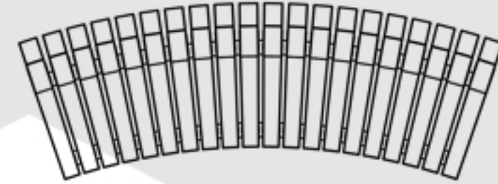
Plateu Seat - Curved Front Radius : 3000mm Front Radius Length : 1980mm Curve Type : Concave Timber 580mm x 120mm Taper : 80mm - 95mm
