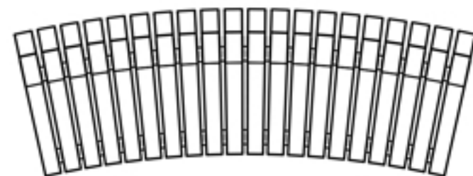
Plateu Seat - Curved Front Radius : 4500mm Front Radius Length : 1980mm Curve Type : Concave Timber 580mm x 120mm Taper : 80mm - 90mm
