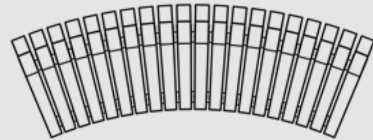
Plateu Seat - Curved Front Radius : 2500mm Front Radius Length : 1980mm Curve Type : Concave Timber 580mm x 120mm Taper : 80mm - 99mm
