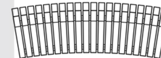
Plateu Seat - Curved Front Radius : 6000mm Front Radius Length : 1980mm Curve Type : Concave Timber 580mm x 120mm Taper : 80mm - 88mm
