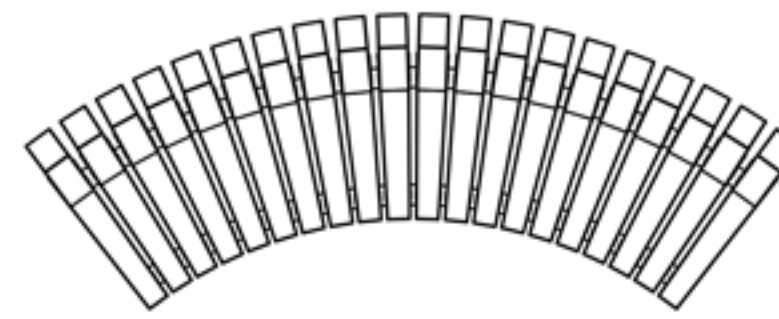
Plateu Seat - Curved Front Radius : 1500mm Front Radius Length : 1980mm Curve Type : Concave Timber 580mm x 120mm Taper : 80mm - 111mm
