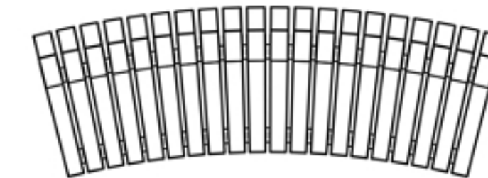
Plateu Seat - Curved Front Radius : 4000mm Front Radius Length : 1980mm Curve Type : Concave Timber 580mm x 120mm Taper : 80mm - 92mm
