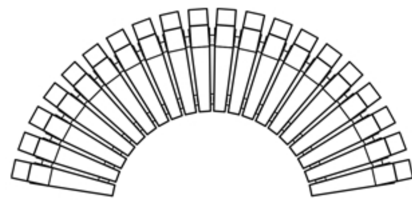
Plateu Seat - Curved Front Radius : 700mm Front Radius Length : 1980mm Curve Type : Concave Timber 580mm x 120mm Taper : 80mm - 146mm
