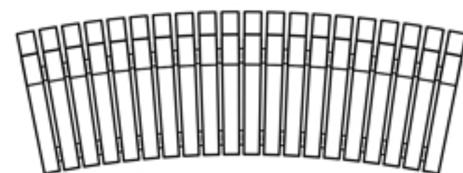
Plateu Seat - Curved Front Radius : 5000mm Front Radius Length : 1980mm Curve Type : Concave Timber 580mm x 120mm Taper : 80mm - 89mm
