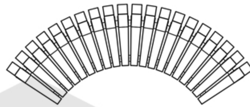
Plateu Seat - Curved Front Radius : 1000mm Front Radius Length : 1980mm Curve Type : Concave Timber 580mm x 120mm Taper : 80mm - 126mm
