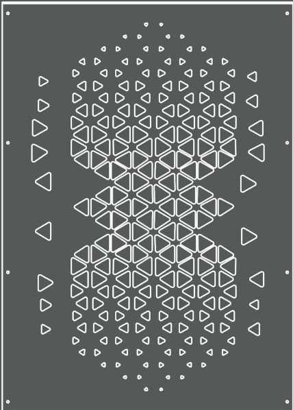
Pattern 4 Steel Percentage - 83% Porosity Percentage - 17%
