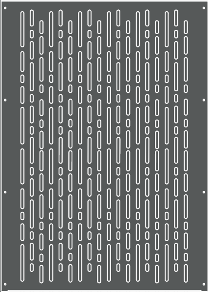
Pattern 2 Steel Percentage - 82% Porosity Percentage - 18%
