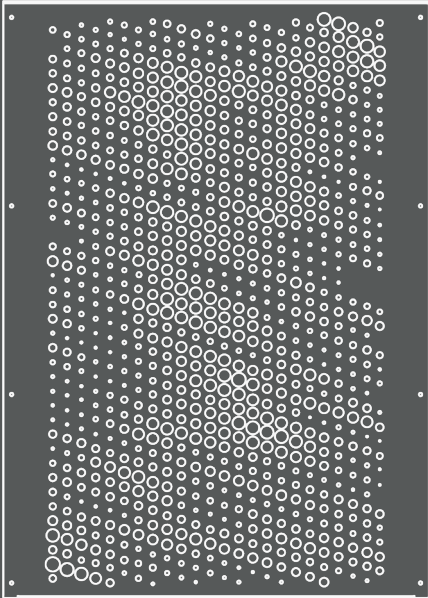
Pattern 1 Steel Percentage - 85% Porosity Percentage - 15%
